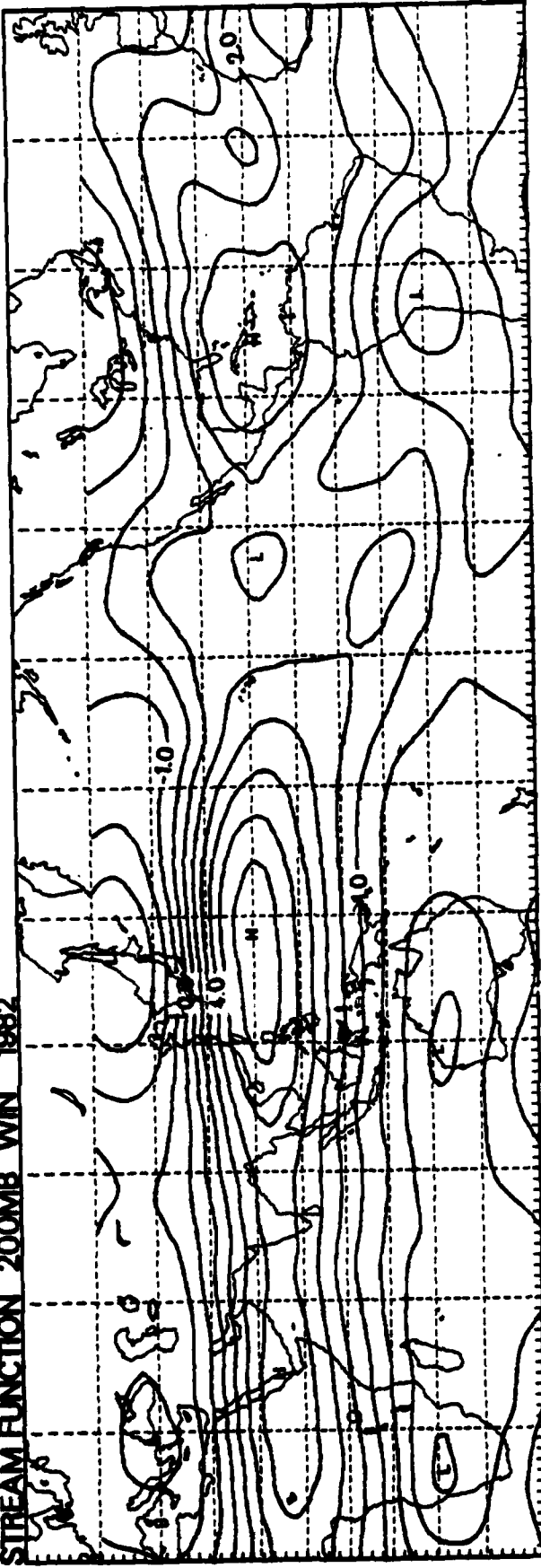
STREAM FUNCTION 200MB WIN 1982
